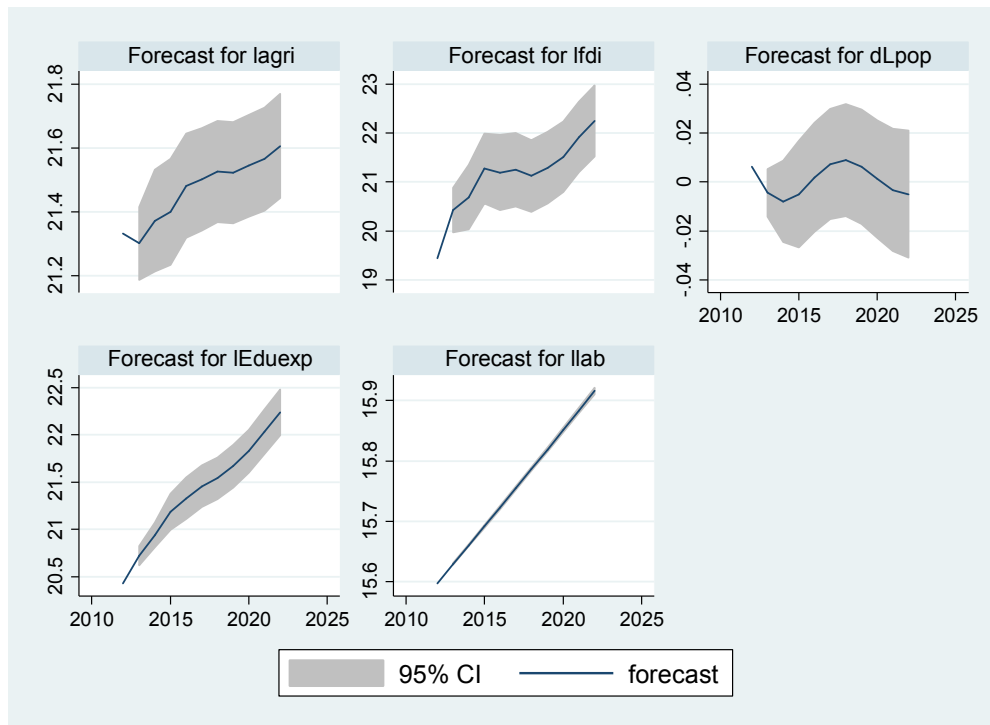
Fig. 1. Graphical representation showing forecasting evolution of each variable in next 10 years
