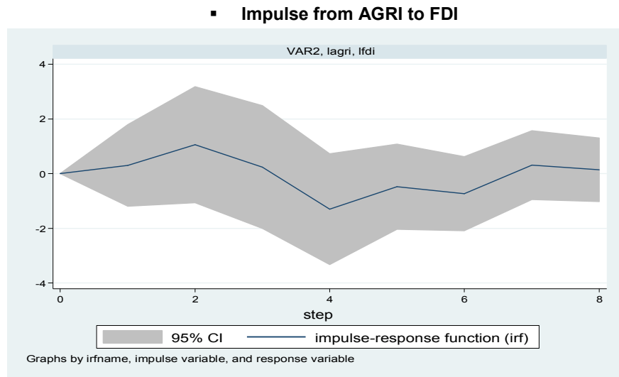
Fig. 3. Graphical representation of impulse response function from AGRI to FDI
