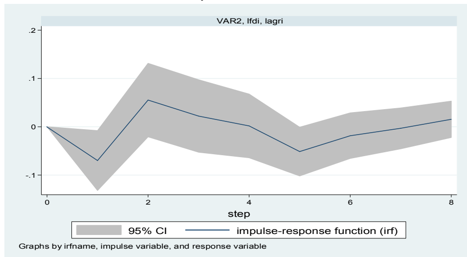
Fig. 2. Graphical representation of impulse response function from FDI to AGRI
