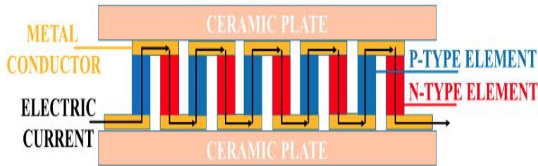
Fig. 4. P-type and N-type elements connected in series
