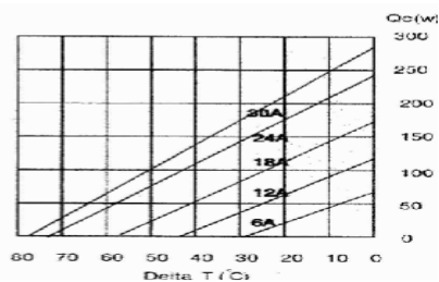
Fig. 8. Specification graph1 for the TEC1-12730 module
