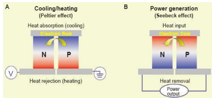
Fig. 1. Thermoelectric principle
