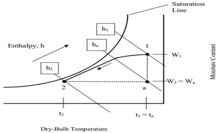
Fig. 6. Psychrometric chart - Cooling and dehumidifying
