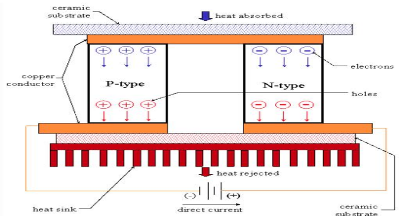
Fig. 3. Principle of thermoelectric module
