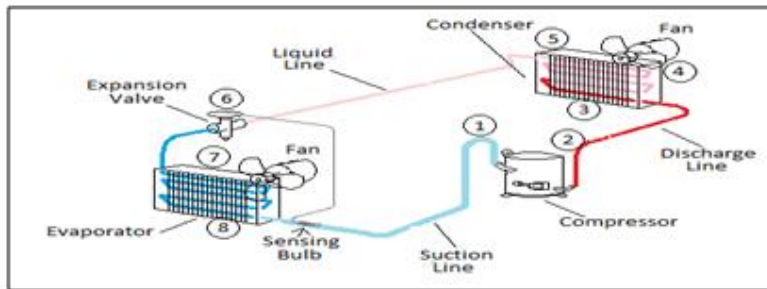
Fig. 2. Refrigeration cycle
