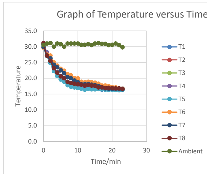
Fig. 13. Graph of temperature/ °C versus Time/min
