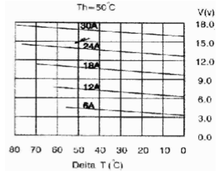
Fig. 9. Specification graph2 for the TEC1-12730 module
