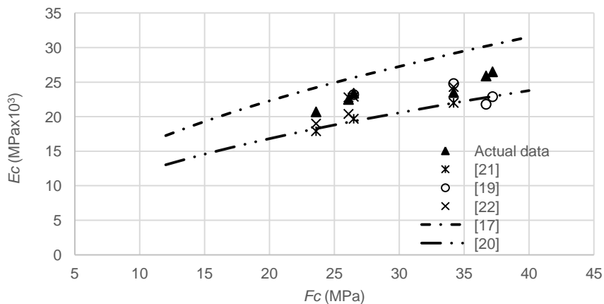
Fig. 6. Modulus of elasticity based on compressive strength
