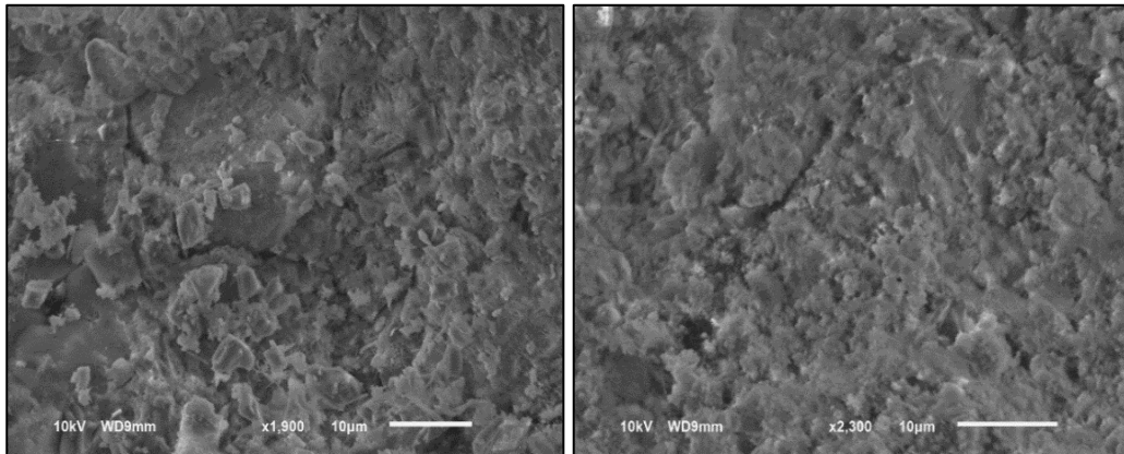
Fig. 7. SEM micrographs of concrete without MWCNTs at 1500x and 2300x
