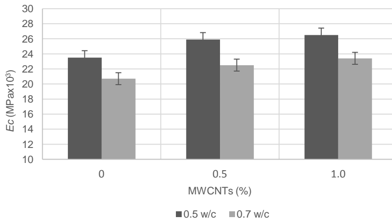
Fig. 4. Modulus of elasticity based on MWCNTs and w/c
