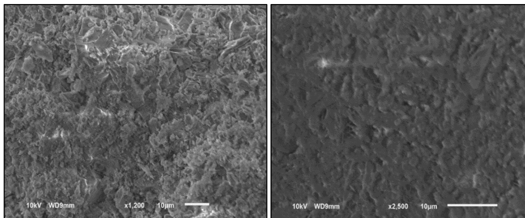
Fig. 8. SEM micrographs of concrete with MWCNTs at 1200x and 2500x
