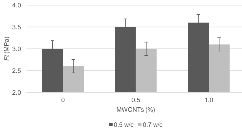
Fig. 3. Splitting tensile strength based on MWCNTs and w/c
