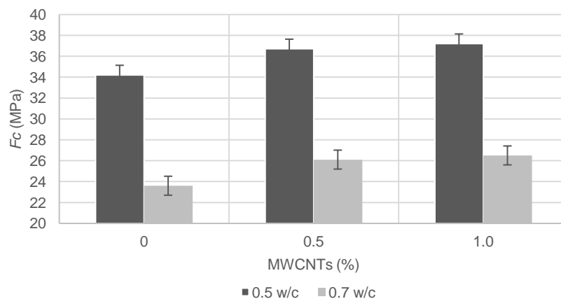
Fig. 2. Compressive strength based on MWCNTs and w/c
