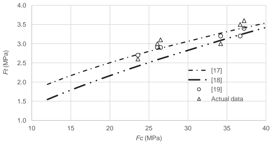
Fig. 5. Splitting tensile strength based on compressive strength
