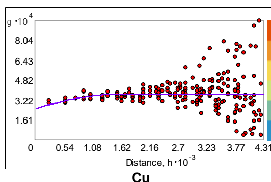
Fig. 2. Semi-variograms and fitted models of soil properties
