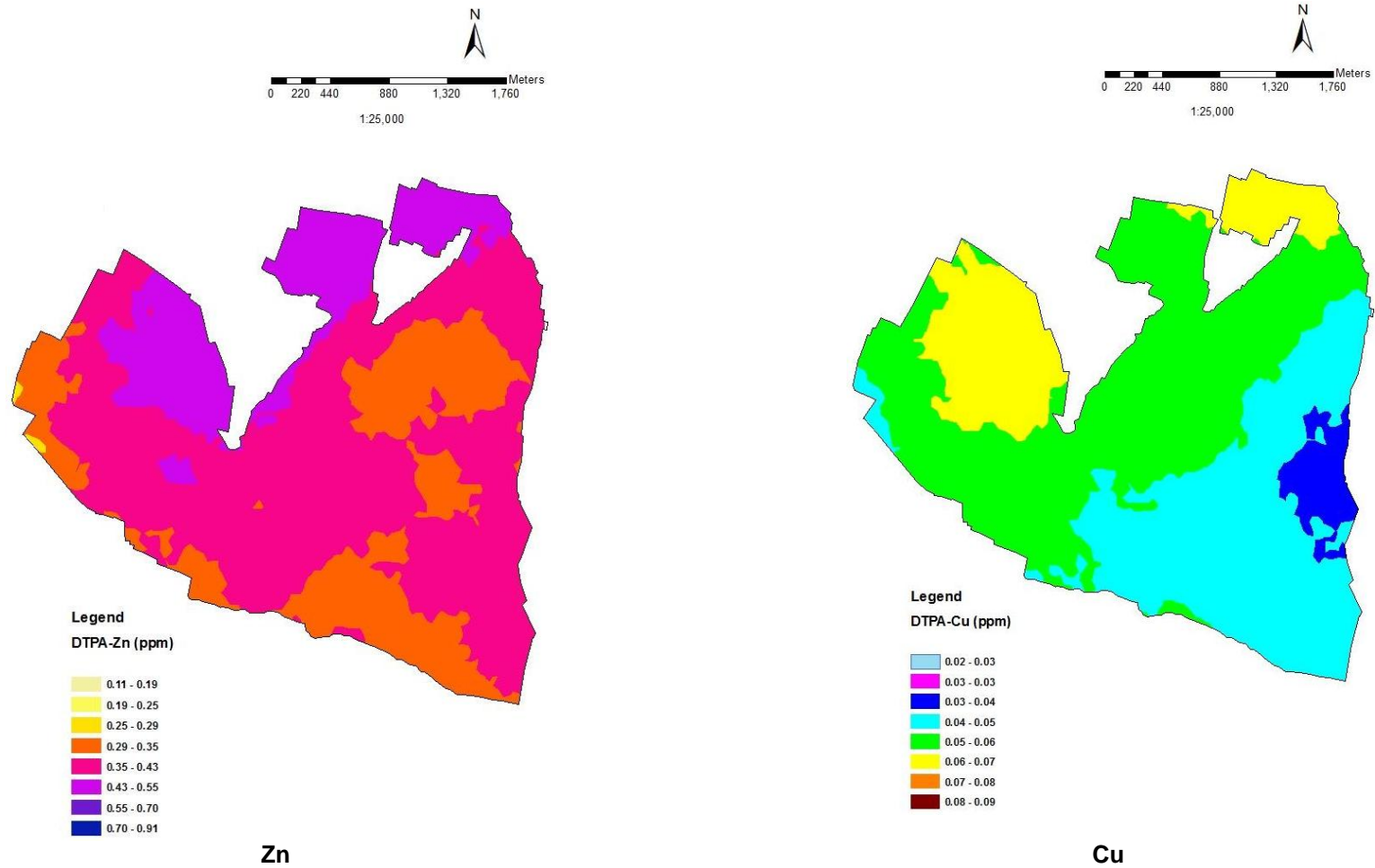
Fig. 3. Map of spatial distribution for eleven soil properties in the study area. EC: soil electrical conductivity; SOC: soil organic carbon AN: available nitrogen; AK: available potassium: AP: available phosphorous AS: Available Sulphur;; Fe, Zn, Mn and Cu are DTPA extractable iron, zinc, manganese and copper in soil
