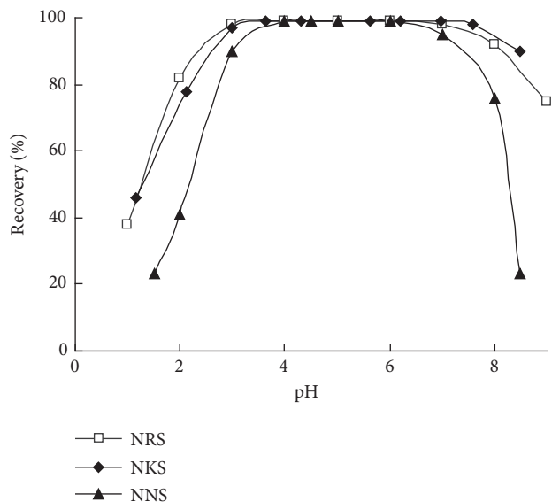
FIGURE 1: Effect of pH on NRS, NKS, and NNS adsorption on SiO 2 -PHMG as a function of pH. m_{ads} = 0.1 g, C_{OR} = 2.65 \cdot 10^{-5} M, sample volume 10 mL, and shaking time 5 min.
