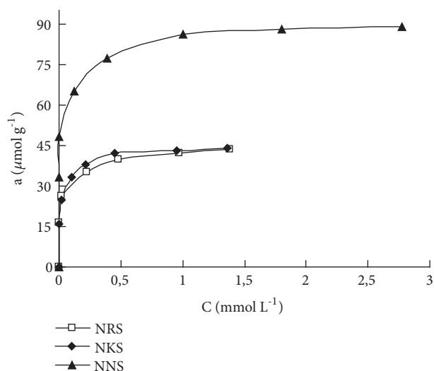
FIGURE 2: Adsorption isotherms of NRS, NKS, and NNS on SiO 2 -PHMG at pH 5. The other conditions are as shown in Figure 1.
