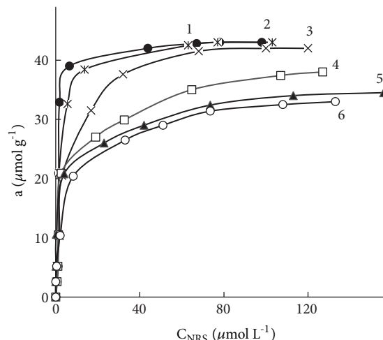
FIGURE 3: Adsorption isotherms of NRS on SiO 2 -PHMG before (1) and after one (2), two (3), three (4), four (5), and five (6) treatments of SiO 2 -PHMG-NRS with 10 mL of hot (50°C) 6 M HCl. Mass of adsorbent-0.1 g, other details of experiments as listed in Figure 1.
