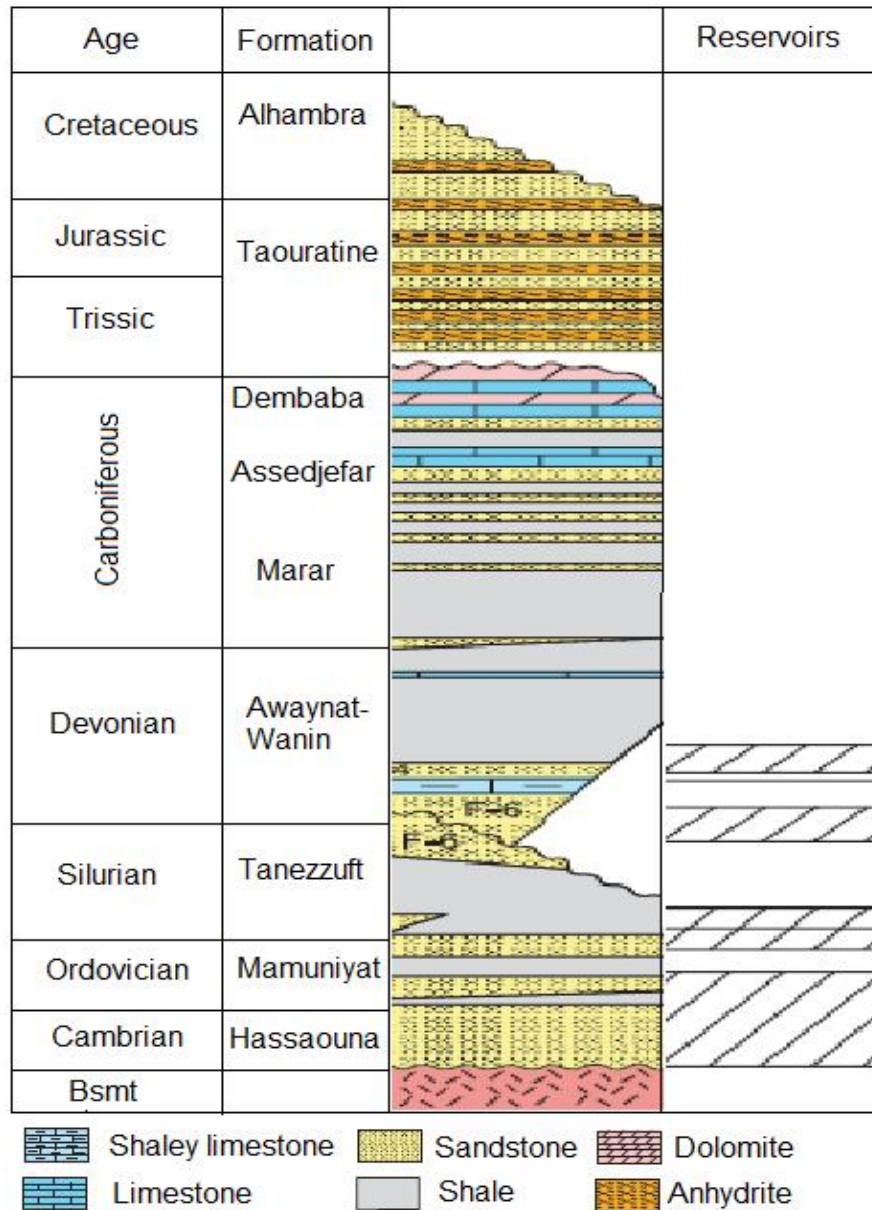
Fig. 2. Stratigraphic column of the Murzuq Basin highlighting the lithology of the formations and the reservoir units. Modified from [4]
