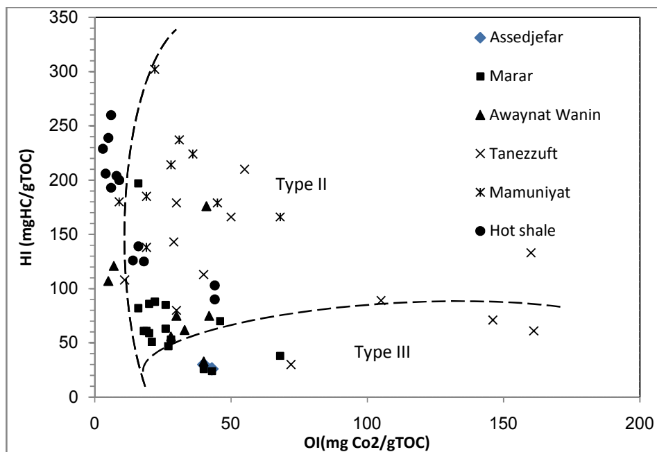
Fig. 3. Plot of hydrogen index (HI) versus oxygen index (OI) illustrating the variation of kerogen type ( II and III) in source rocks of the studied fields [10]
