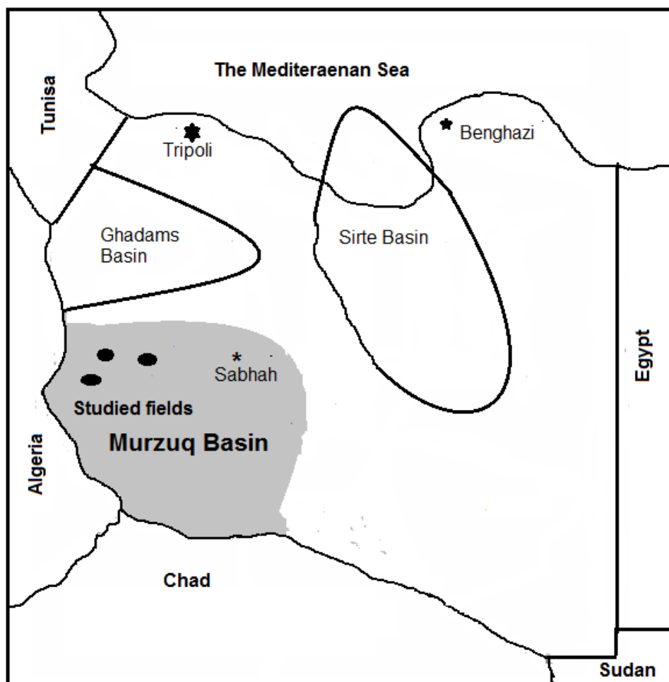
Fig. 1. Map shows the location of the Murzuq Basin and studied fields Modified from Hallett D. 2002 and Abogllila et al. 2010
