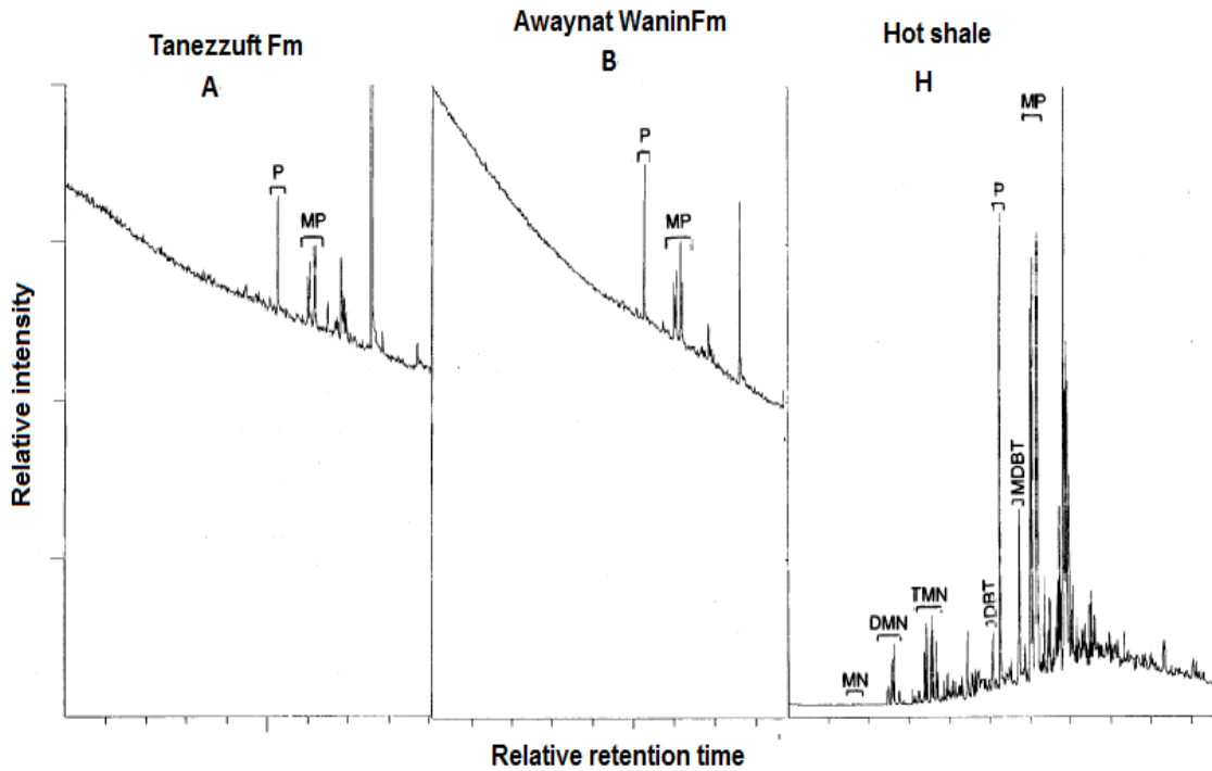
Fig. 5. Aromatic fraction gas chromatography - mass spectrometry of three selected formation from three fields, peak identification in Table 3
