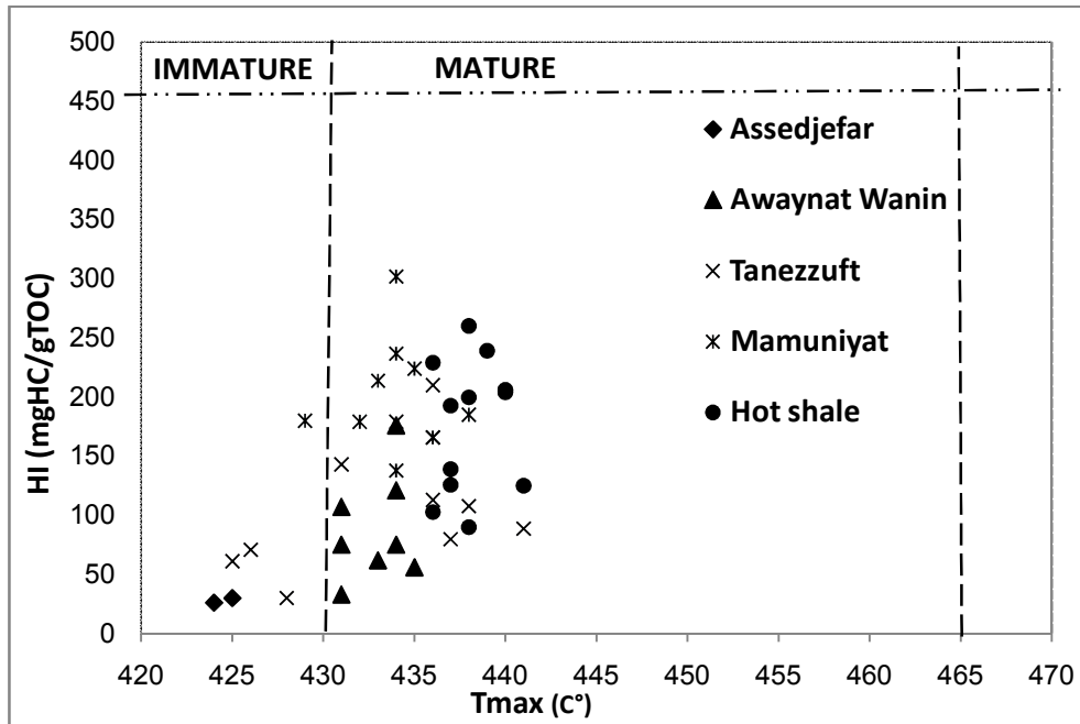
Fig. 4. A plot of HI vs Tmax from Rock-Eval pyrolysis showing position of various samples from three fields, Murzuq Basin [10]
